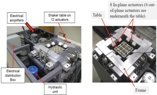
Figure 7- Multi-axial ED Shaker at CALCE
