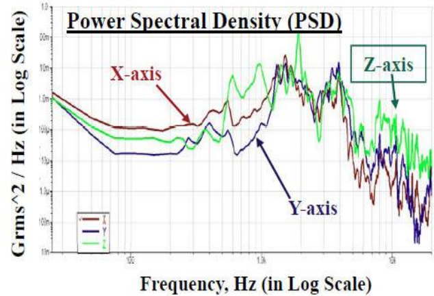
Figure 5- PSD in RS Shaker (Choi et al. , 2009)
