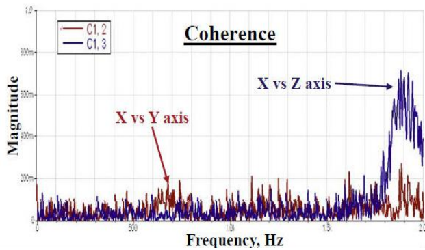
Figure 9- Coherence in Multi-axial Shaker (Choi et al., 2009)
